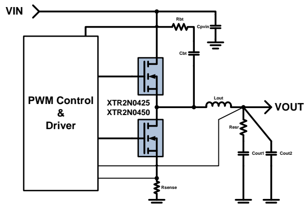
Step-down DC-DC Converter
