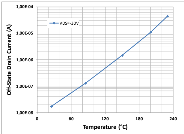
Figure 7. Off-State Drain Current ( I_{oss} ) vs Case Temperature. V_{DS}=-30V , V_{GS}=0V .
